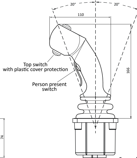
Forward orientation indent (orientation mark, Y axis)
