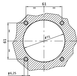
Panel mounting details
