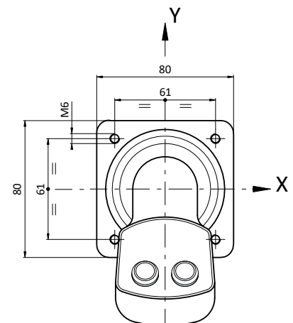
Panel mounting details
