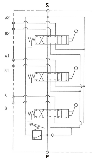
3 leve/levers
