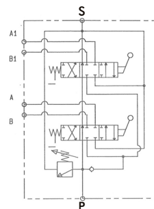
2 leve/levers
